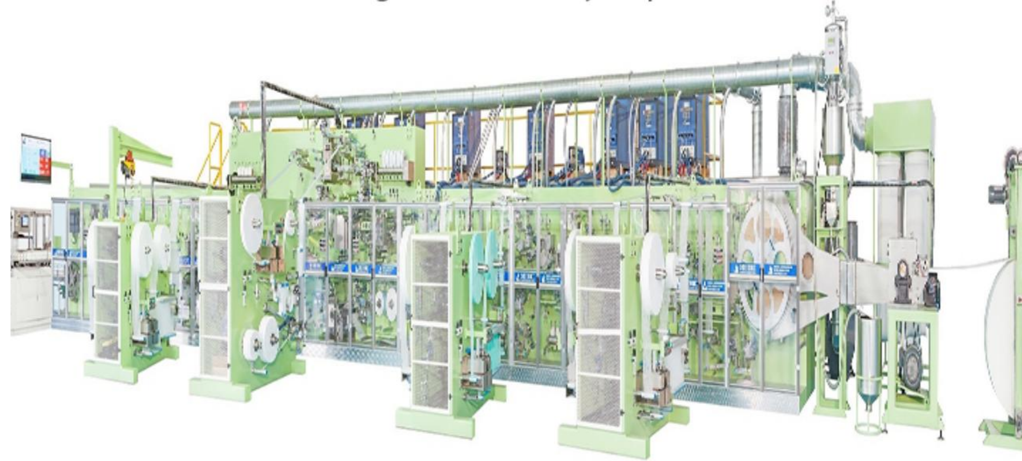
Full Servo Big Waistband Baby Diaper Production Line
